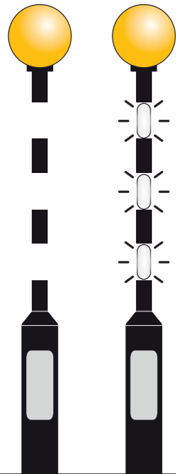
Belisha Beacon Pedestrian Post Painted or Retroreflective Bands
